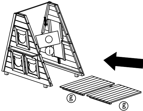
step 3: put in floor and partition.
