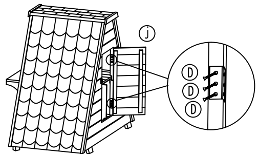
Step 6: set up back side door.(finished)
