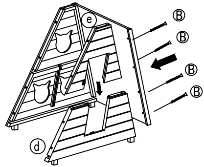
step 2: set up back up and down panels, and set up right side panel.
