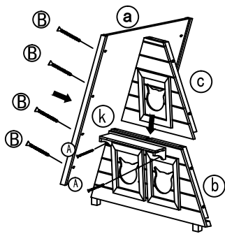
step 1: set up front up and down panels, and set up balcony and front down panel.
